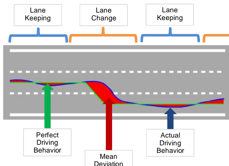
Illustration 2: Measurement of driving behaviour. The green line indicates the ideal path, the blue line shows an example of a test driver’s path. The deviation between the blue line and the green line (shown in red) describes the extent of the distraction. A further distinction can be made between the lane change and lane keeping phases.
